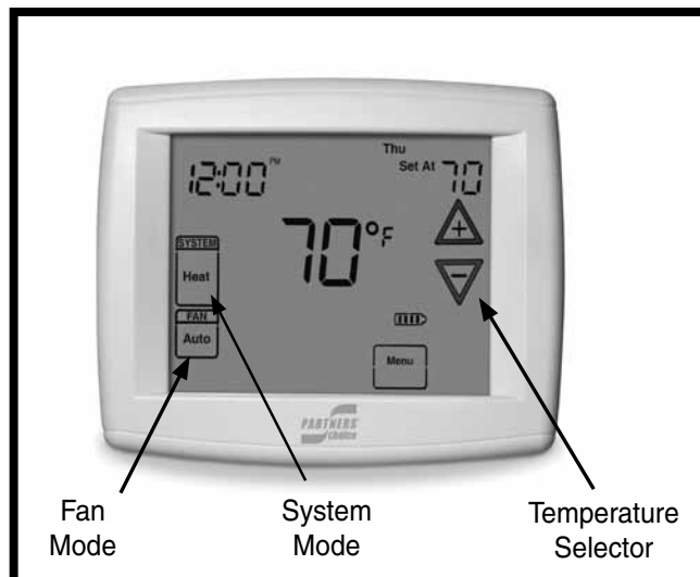
Figure 1. Digital Thermostat
